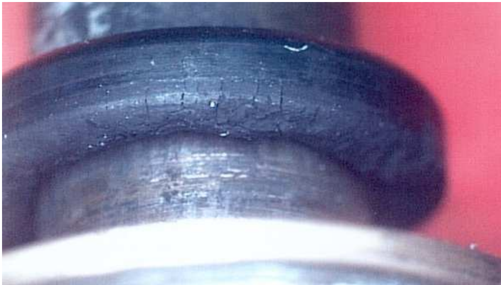
Photo 6: NBR O-Ring after excessive thermal exposure, with severe cracking and flattening.
