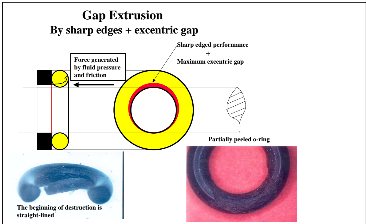
Photo 10: Damage from a sharp edged backup ring at relatively low pressures (<50 bar).
