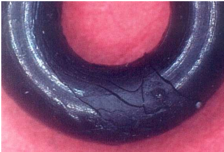
Photo 1: Extreme flow lines; during injection if mold flow runners are too long or mold temperature too high, the material scorches.
