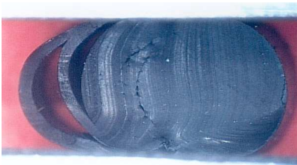
Photo 2: Internal splits, that propagate through the O-Ring during service. The probable cause most likely the use of scorched material (expired shelf life).
