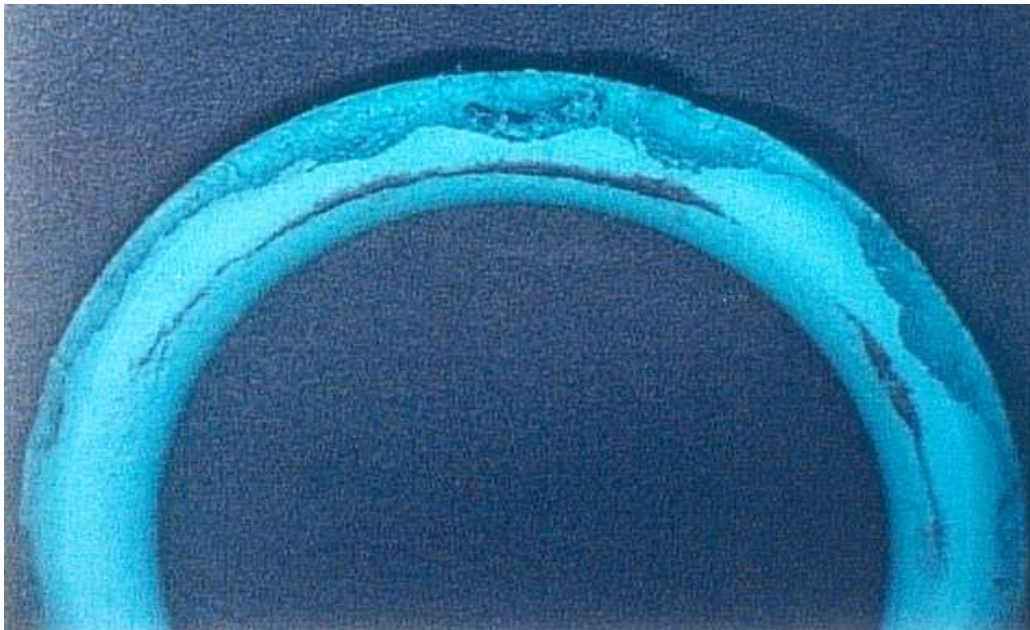
Photo 9: Damaged O-Ring resulting from sharp corners and high pressures (ca. 250 bar).
