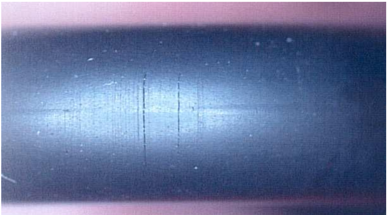
Photo 4: O-Ring damage from passing over guide chamfer.
