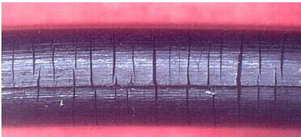
Photo 12: Splits on the fluid side are typical characteristics of chemical attack.
