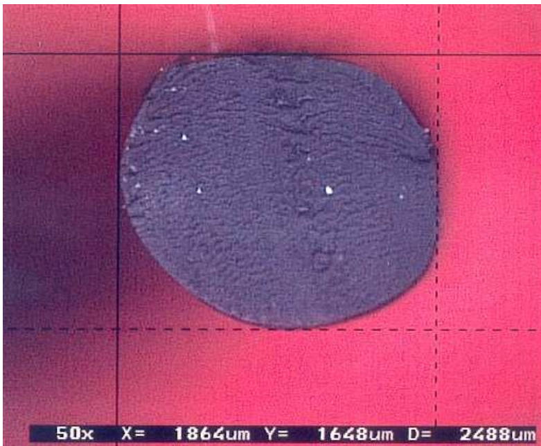
Photo 11: Single abraided flat surface on O-Ring (static seal)
